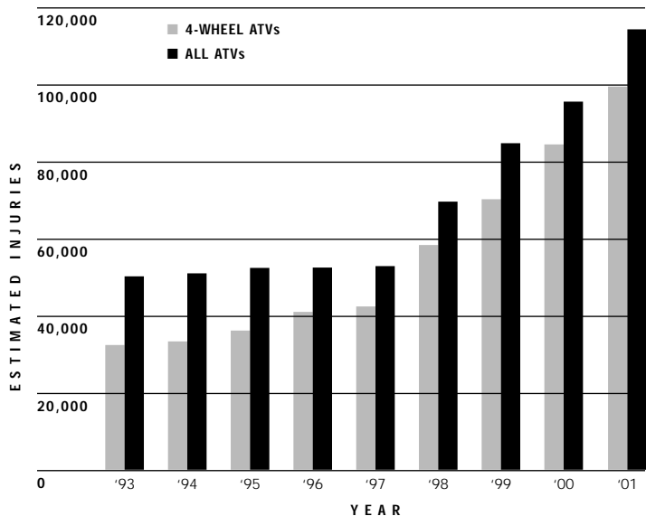
FIGURE 2 ATV Injuries
