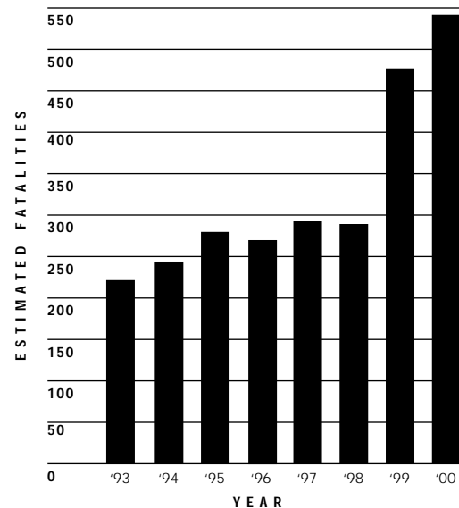
FIGURE 3 ATV Fatalities
